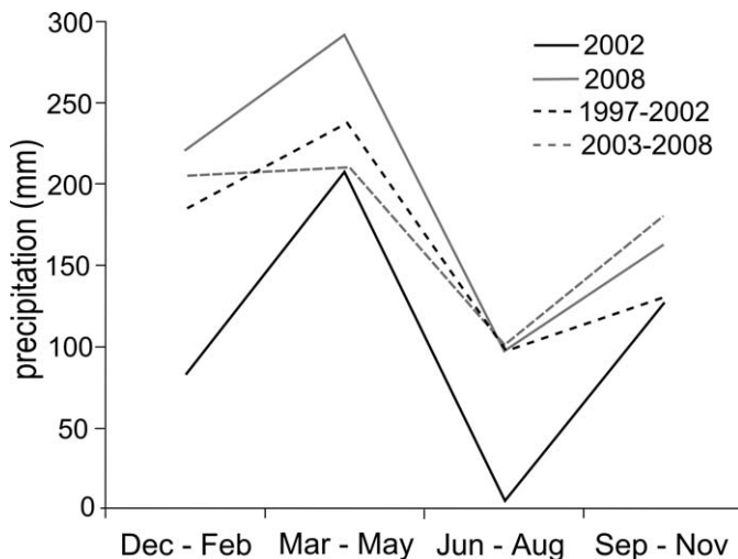
Figure 2. Mean precipitation (mm) for vegetation sampling years (2002, 2008) and 6-yr periods prior to and including sampling years from the South Pass Snotel site (~ 24 km from center of study area) for 3-mo increments approximating winter, spring, summer and autumn.
